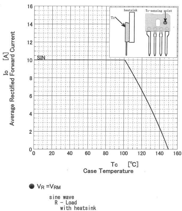
Derating Curve
