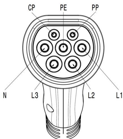
Pin assignment of the vehicle connector
