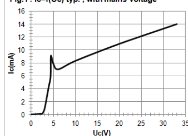
Fig.1 : I c =f(U c ) typ. , with mains voltage
