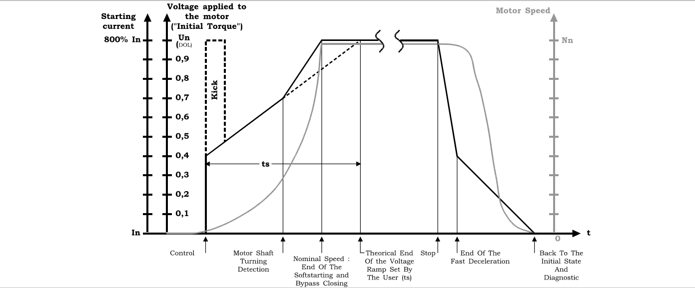
Fig. 3 DESCRIPTION OF THE DIFFERENT SETTING PARAMETERS
