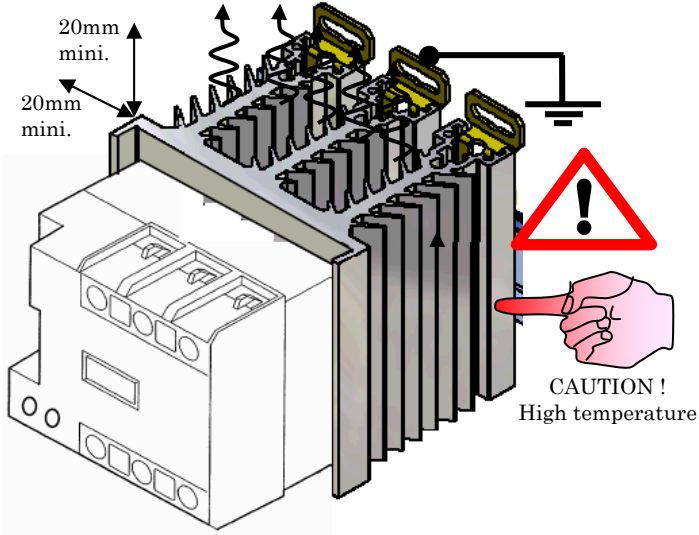
Fig. 24 Mounting With Screws
