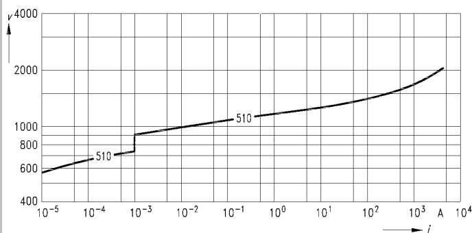
Overvoltage Protection Characteristic (Varistors)
