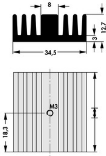
SK 126 25 TO 220 SK 126 37,5 TO 220
