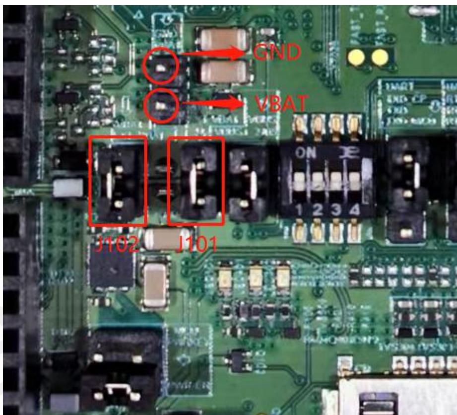
Figure 7: Power supply test points (VBAT GND)
