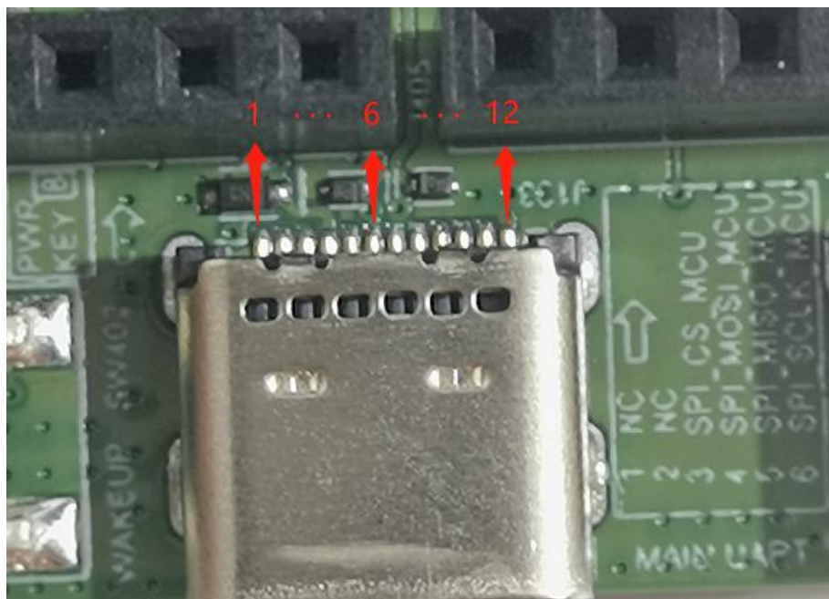
Figure 11: The definition of the Type-C interface (J103)
