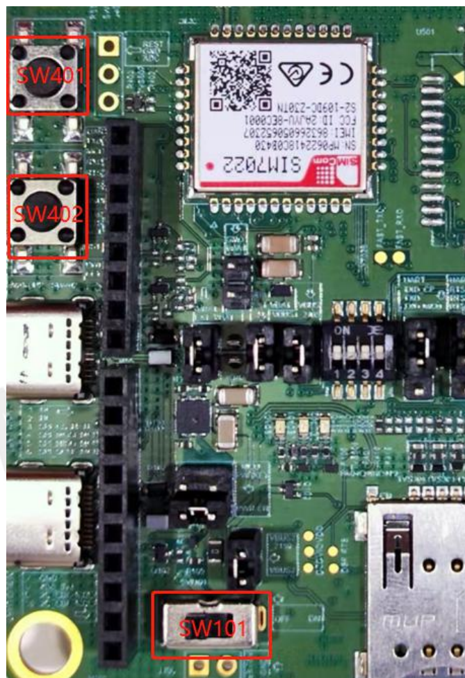
Figure 13: Switch and Buttons
