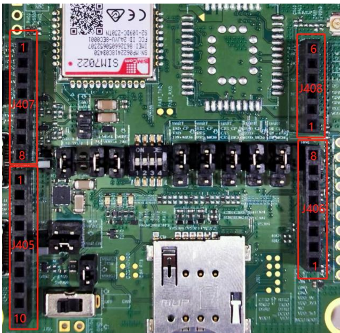
Figure 14: Arduino interface on the EVB
