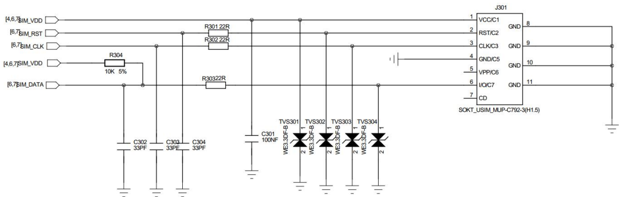
Figure 8: The (U)SIM reference design
