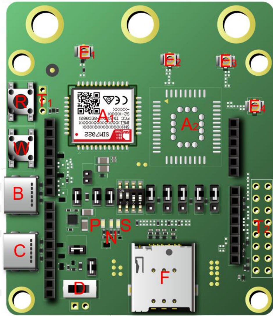
Figure 1: The top view of NB-EVB
