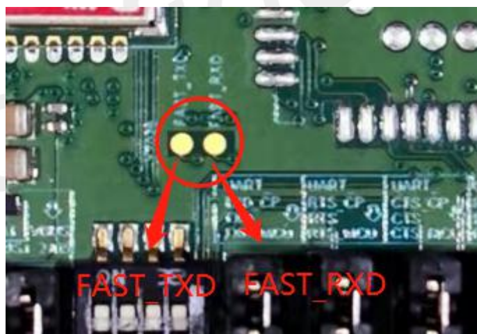
Figure 26: The test point of the FAST_TXD and FAST_RXD
