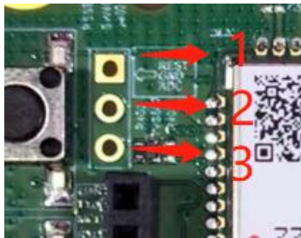
Figure 25: The test point of the J402
