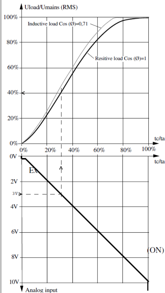
Fig.1 Transfer characteristic :
