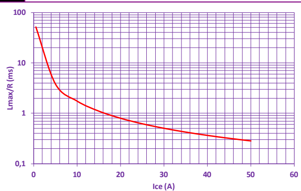
MAXIMUM TIME CONSTANT WITH RL INDUCTIVE LOAD
