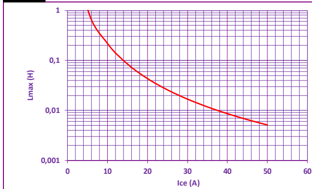
MAXIMUM TOTAL INDUCTANCE (LOAD+LINE) ADMISSIBLE BY THE IGBT
