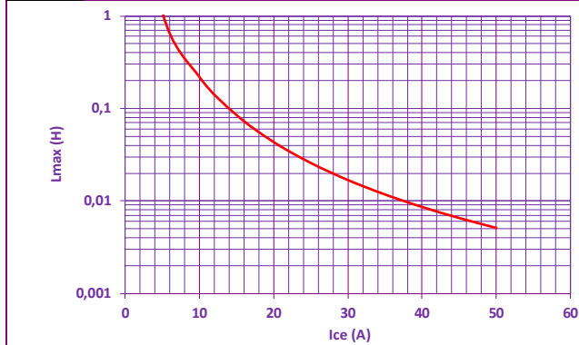
Fig. 9 MAXIMUN TOTAL INDUCTANCE (LOAD+LINE) ADMISSIBLE BY THE IGBT
