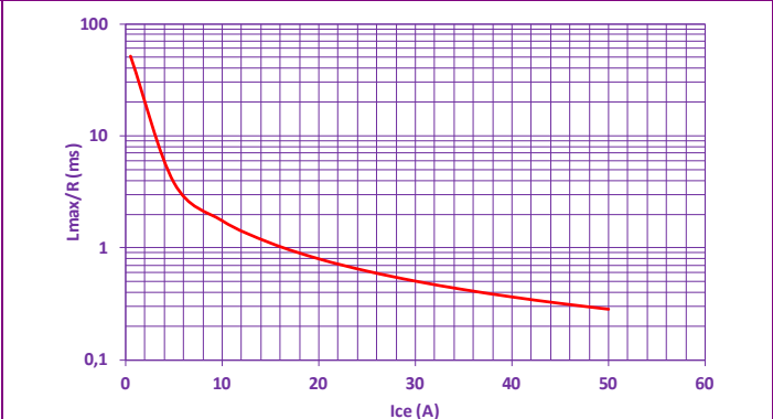
Fig. 10 MAXIMUN TIME CONSTANT WITH RL INDUCTIVE LOAD
