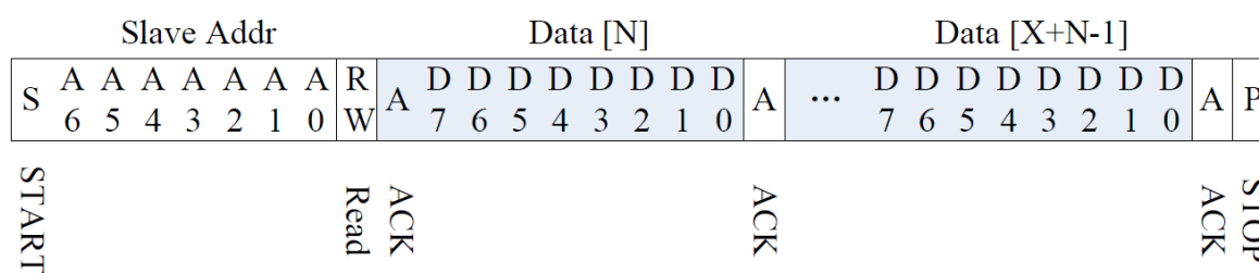
Figure 12. Read X bytes from I2C Slave
