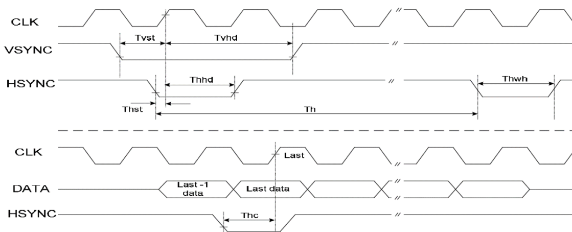
Figure 8. Timing diagram
