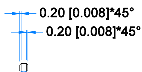
DETAIL C SCALE 4:1
