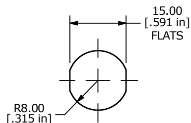
PANEL MOUNTING
