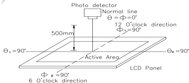
Fig 11.2. Optical measurement system setup
