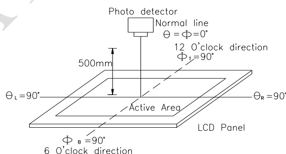
Fig. 10.2. Optical measurement system setup
