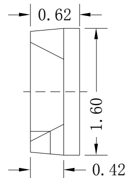
Fig.1-2 Side view 侧面视图
