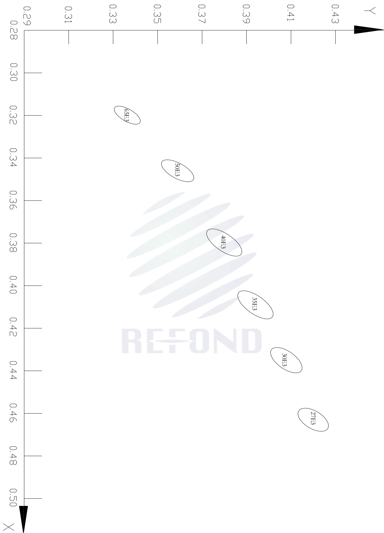
Fig 1-6-2 The C.I.E Chromaticity Diagram CIE色度图
