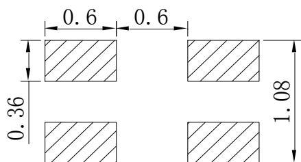
Fig.1-5 Soldering patterns 推荐焊盘
