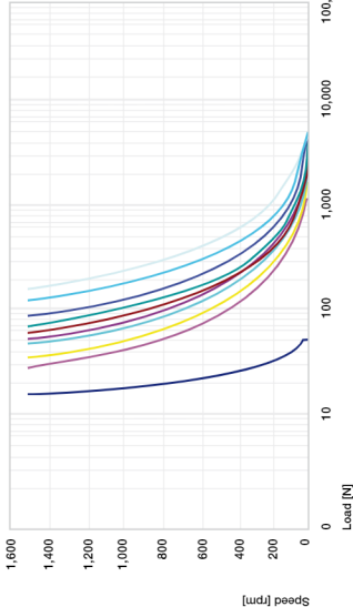
Diagram 10: Maximum dynamic load for lead screw drives with 100% ESD
