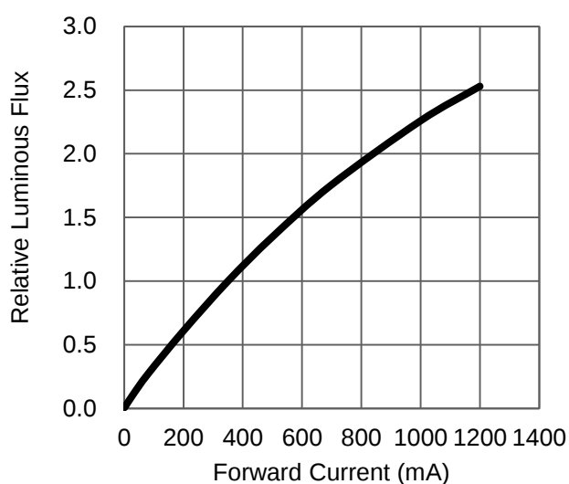
Fig 2. Relative Luminous Flux vs. Forward Current.
