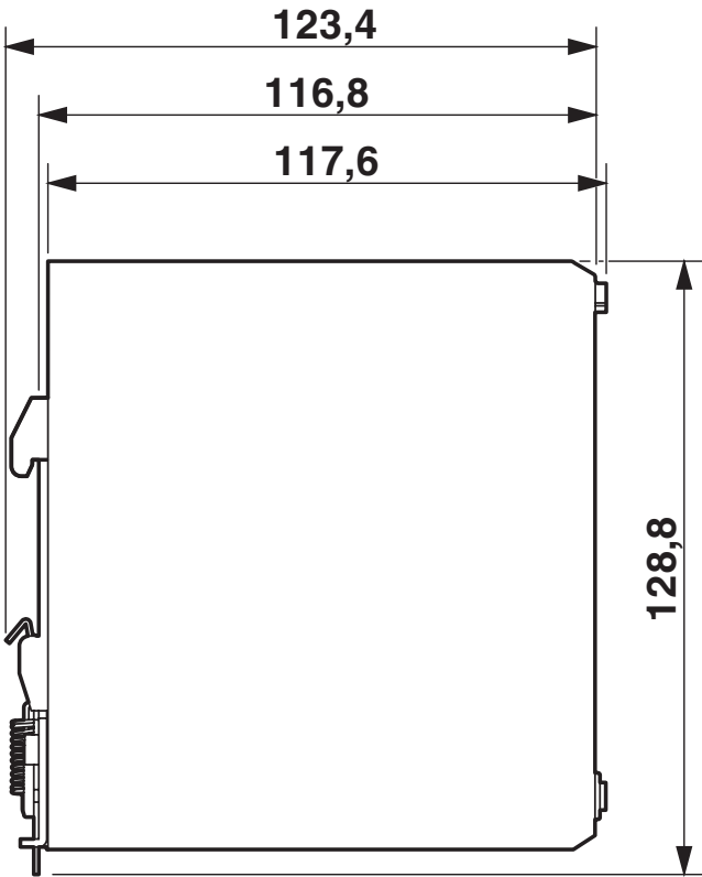
Dimensional drawing
