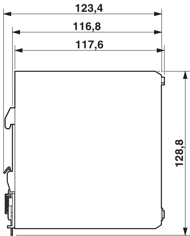
Dimensional drawing
