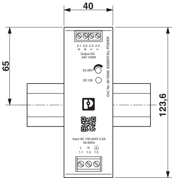
Dimensional drawing
