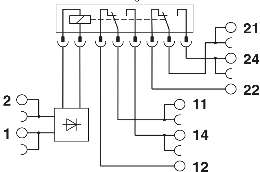
Circuit diagram
