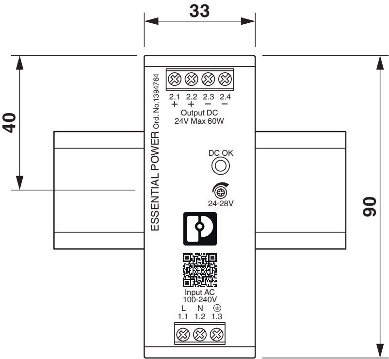
Dimensional drawing
