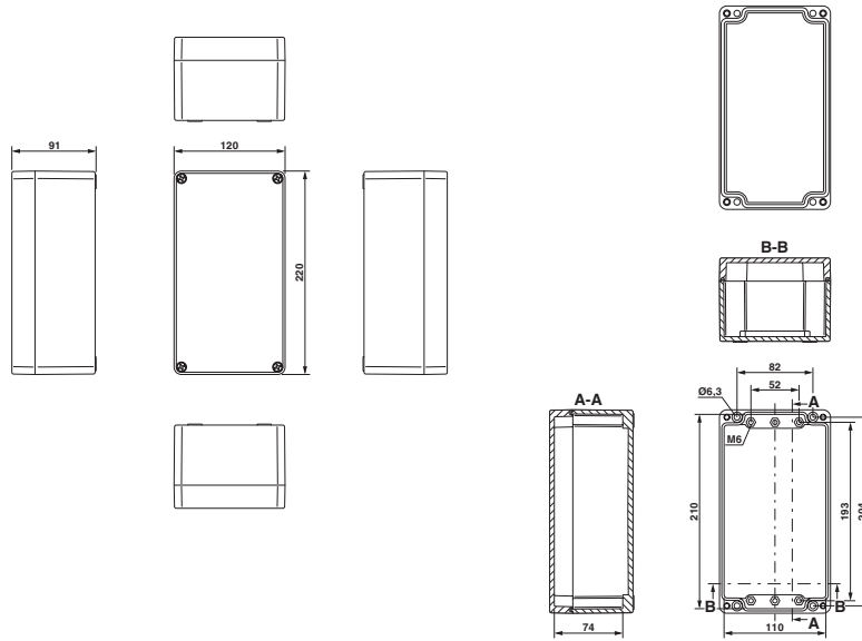
Dimensional drawing
