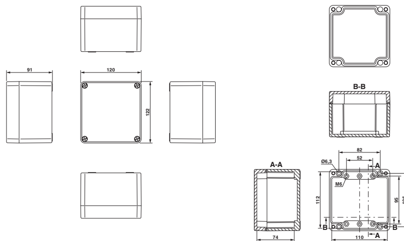
Dimensional drawing
