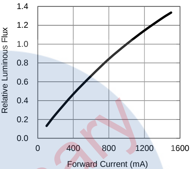
Fig 6. Forward Current vs. Relative Luminous Flux at T j =25°C.
