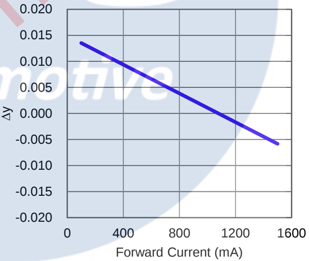
Fig 8. Forward Current vs. Chromaticity Coordinate Δy at T j =25°C.
