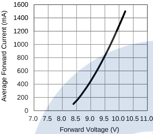
Fig 5. Forward Voltage vs. Forward Current at T j =25°C.
