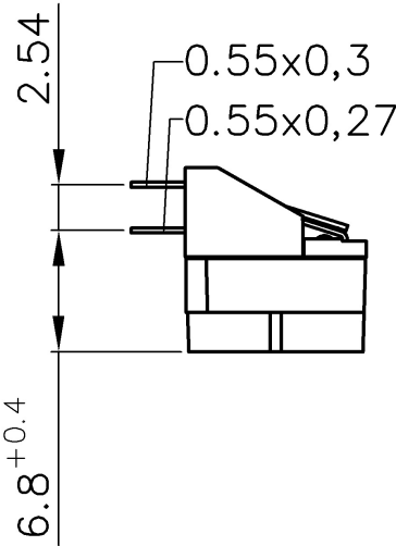
Left angular 2.54 mm
