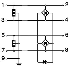
4-pole version
