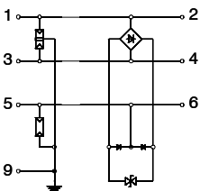
3-pole version
