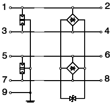
4-pole version
