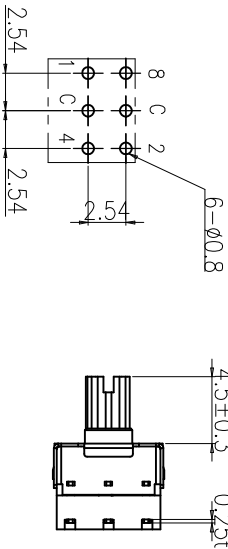
P.C.B. DIMENSION (Top View)
