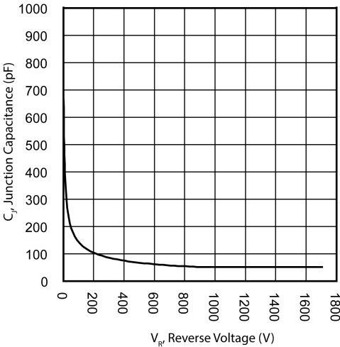
Figure 7 • Junction Capacitance vs. V R
