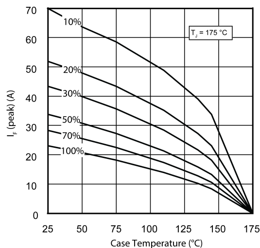
Figure 3 • Max. Forward Current vs. Case Temp.
