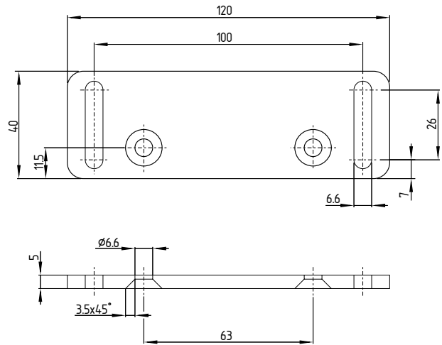
Mounting plate, part of the mounting set MS-AZM400 (available as accessory)
