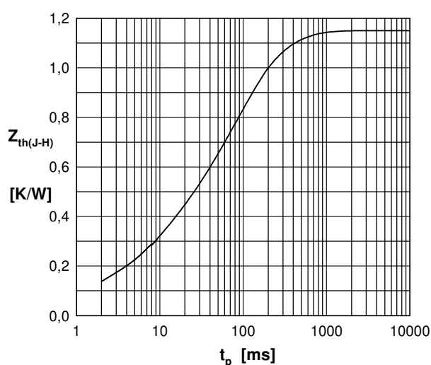
Fig. 18 Typical transient thermal impedance
