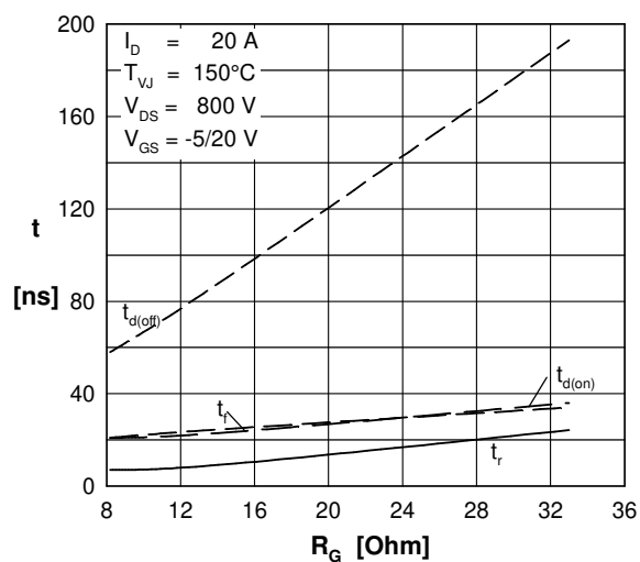
Fig. 16 Typical switching time versus external gate resistor
