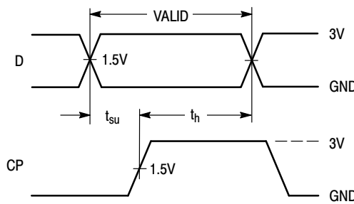
Figure 5. Switching Waveform
