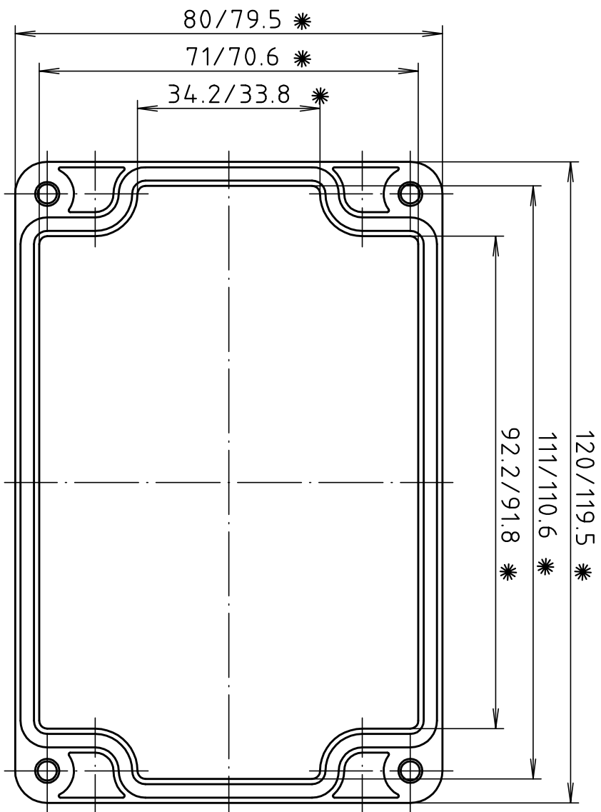
Deckel/lid
