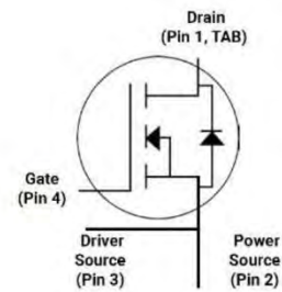
TO-247-4L Pin definition
