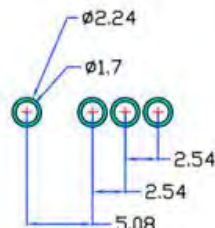
Recommended Solder Pad Layout
