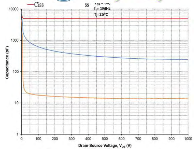
Figure 8. Capacitances vs. Drain-Source Voltage (0-1000V)
