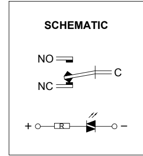
SINGLE-BREAKPOINT QUICK- ACTING CONTACT SWITCHES WITH THREE TERMINALS
