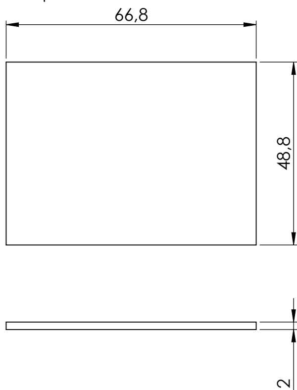
Front panel
