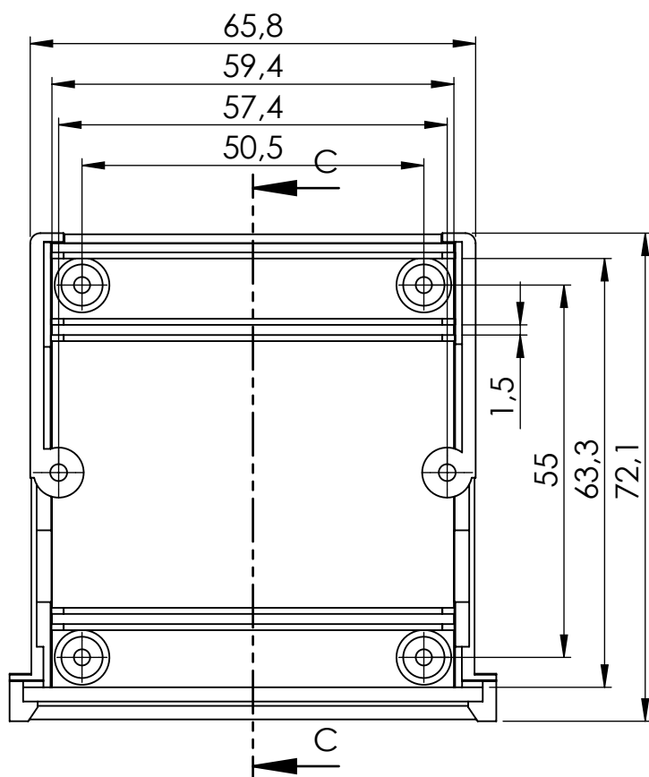
Rear panel
