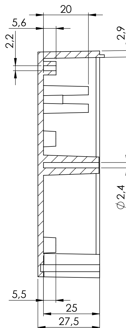
SECTION B-B
