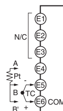
Temperature Indicator K3HB-H
