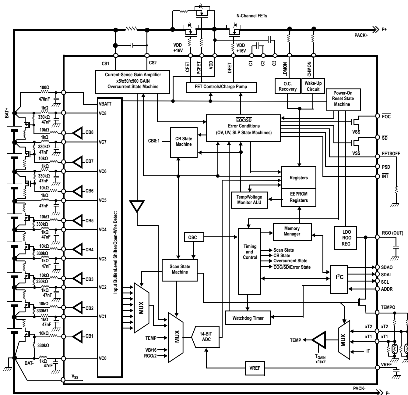
Figure 2. Block Diagram
