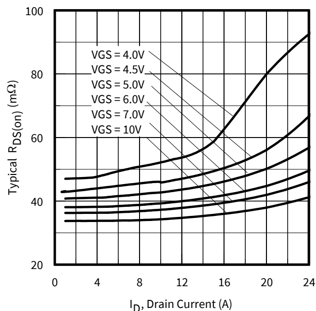
Figure 2 Typical On-Resistance vs. Drain Current
