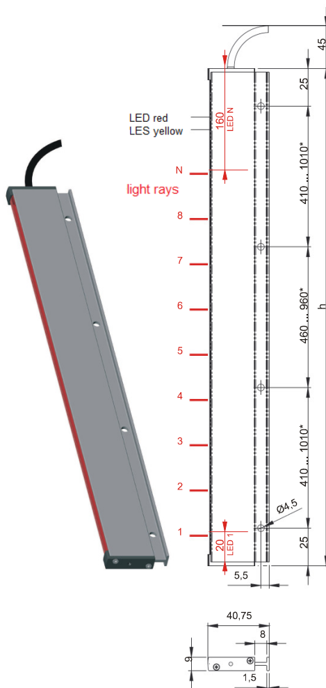
bracket mounting
