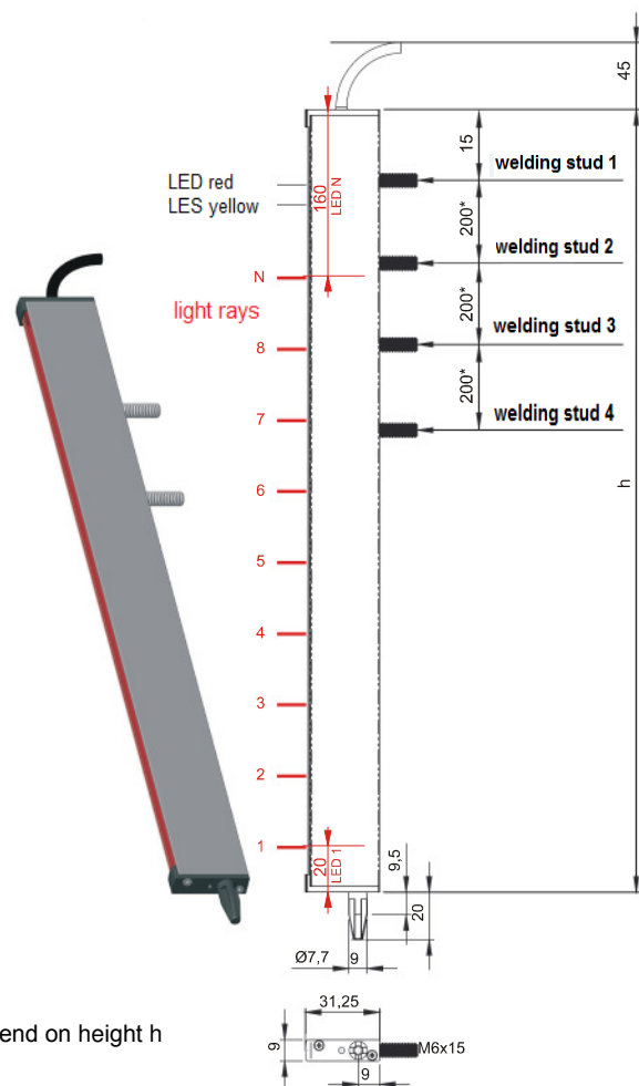
bolt mounting
