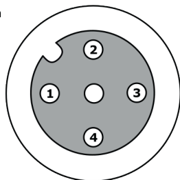
female connection
