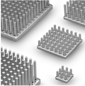
Heatsinks and active heatsinks for processors>Pin heatsinks 36 x 36 x 30 mm, pin heatsinks quadratic
