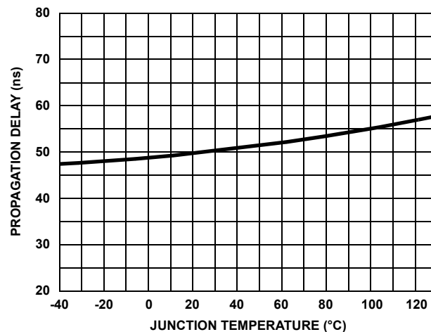
FIGURE 17. DISABLE TO LOWER ENABLE TDPLH PROPAGATION DELAY vs TEMPERATURE
