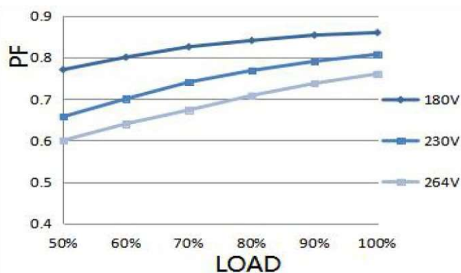
PF CURVE
