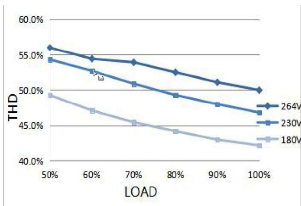
THD CURVE
