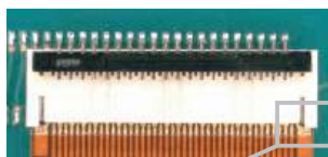
Correct FPC Insertion
