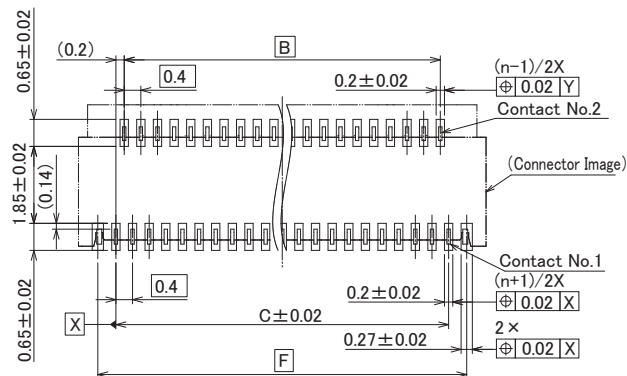
Recommended PCB Mounting Pattern
