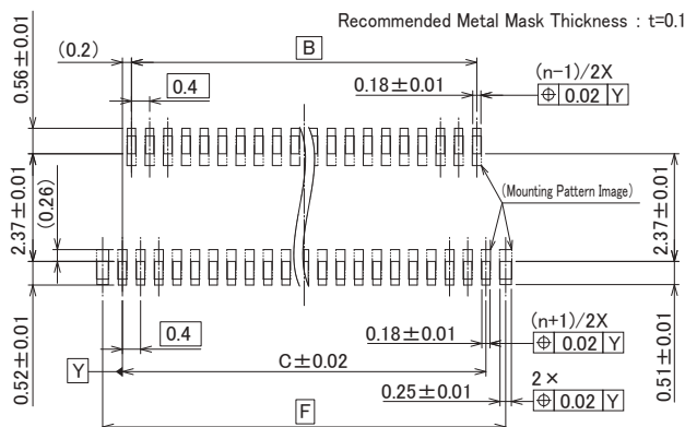
Recommended Metal Mask Dimension
